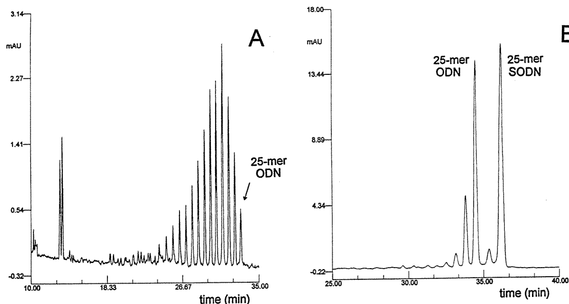
Fig. 4. Digestion of Oligomer 1 in (A) 3'-exonuclease solution and (B) 3'-exonuclease solution in the presence of Oligomer 6. Reaction conditions were identical; the time of reaction in both cases was 115 min. For details see text and Section 2.
