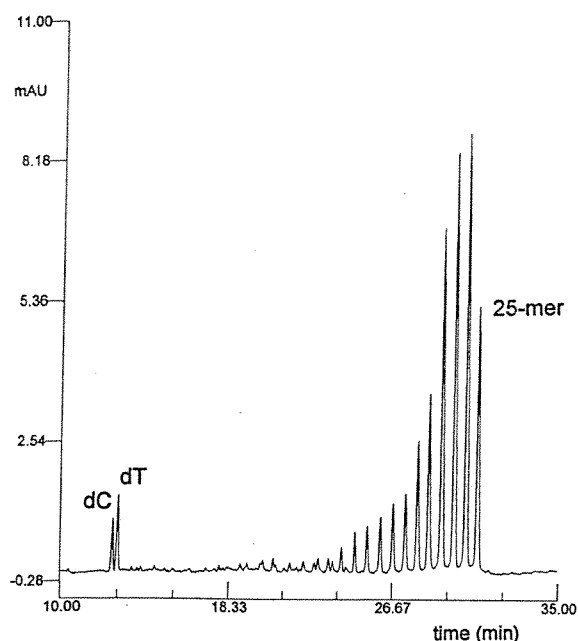
Fig. 1. Separation of ODN (Oligomer 1) metabolites of 3'-enzymatic hydrolysis. Reaction time was 55 min. Peaks dC and dT (12.55 and 12.81 min) correlate with the 5'-mononucleotides, deoxycytidine and deoxythymidine 5'-monophosphate nucleotides, respectively. Migration order was established by spiking the solution with the appropriate mononucleotides. For conditions see the experimental section.
